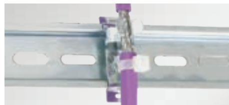
EMC shield clamps for 35 mm top hat DIN rails with/without strain relief function
