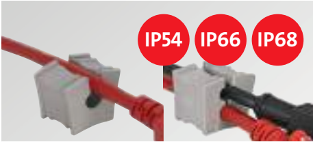
KT cable grommets split, for cables with and without connectors for cable diameters 1 – 35 mm 76, 80
