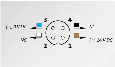
M12 connector female (SC versions)
