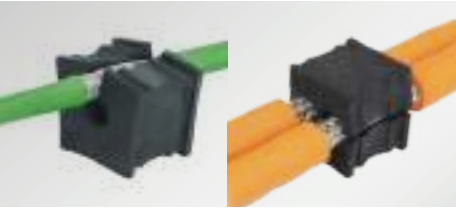
Split EMC grommets small, single and multi for cables with and without connectors for cable diameters 2 to 16 mm EMC-KT 280
