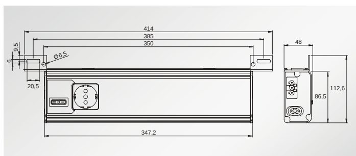
Version without motion sensor, with socket for door operated switch
