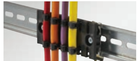
Strain relief plates for 35 mm top hat DIN rail snap mount
